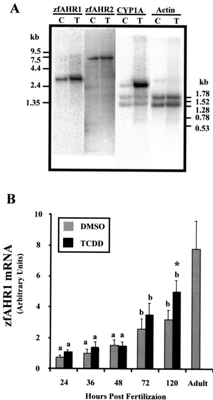
Fig. 3. Presence of zfAHR1 , zfAHR2 , and zfCYP1A mRNAs in zebrafish larva. A, Northern blot of poly(A + ) mRNA from 120-hpf whole zebrafish larva. Embryos were treated with a water-borne LC 100 (1.55 μM) concentration of TCDD within 3 h of fertilization. Five micrograms of mRNA was resolved in each lane. Molecular mass markers, indicated on the left and right of the images in kilobases (kb) confirmed estimated size of each specific band. The blot was sequentially probed with random-primed cDNA probes for zfAHR1 , zfAHR2 , zfCYP1A , and rat β-actin. Abundance of message was detected by exposure to phosphor screen. Exposure times for the probes were zfAHR1 (4 days), zfAHR2 (2 days), zfCYP1A (1 day), and β-actin (12 h). B, time course of zfAHR1 mRNA expression in vehicle (control) and TCDD-exposed embryos by quantitative real-time PCR. Samples were run concurrently with standard curves derived from plasmid cDNA dilutions. zfAHR1 expression values were normalized to actin mRNA levels. The height of each bar represents the mean ± S.E.M. (n = 5). * indicates significantly different from control at the same time (p < 0.05). a and b indicate two groups with similar mRNA abundance.
