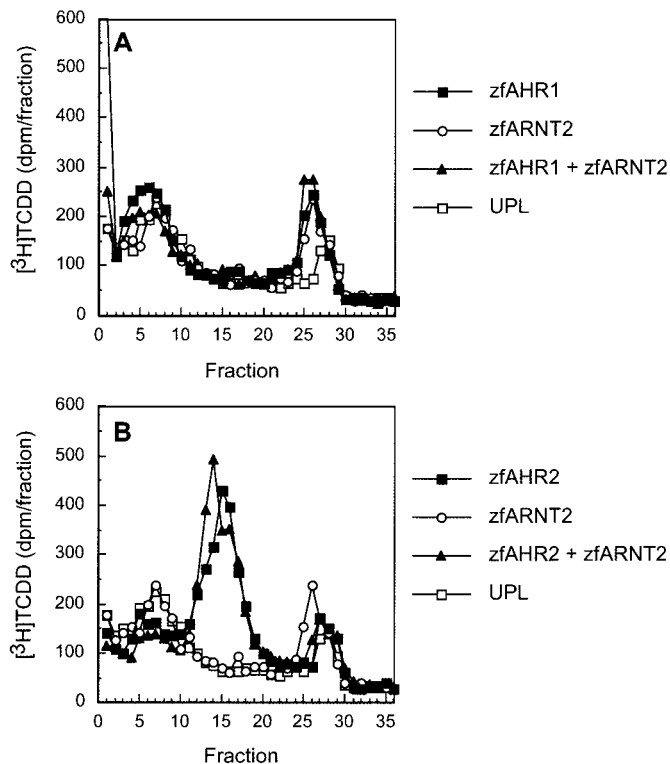
Fig. 9. Analysis of [ 3 H]TCDD-specific binding after coexpression of zfAHR1, zfAHR2, and zfARNT2. zfAHR1 (A) or zfAHR2 (B) was expressed singly or coexpressed with zfARNT2b as described for the DNA binding assays. After in vitro transcription and translation (90 min at 30°C) in the presence of 5 nM [ 3 H]TCDD, reactions were analyzed by velocity sedimentation as described in the legend to Fig. 8.
