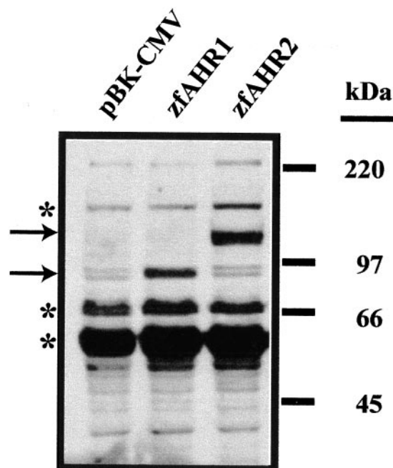
Fig. 7. Western-blot analysis detecting the presence of zfAHR1FLAG and zfAHR2FLAG in COS-7 cell lysate. COS-7 cells were transiently transfected with expression constructs for zfAHR1FLAG, zfAHR2FLAG, or an empty vector (pBKCMV). Lysate was harvested after 30 h. Twenty micrograms of lysate was resolved on an 8% SDS PAGE gel and transferred to nitrocellulose membrane for Western analysis. The membrane was incubated with 2 mg/ml anti-FLAG antibody followed by goat anti-mouse horseradish peroxidase (1:5000). Enhanced chemiluminescence was used to visualize the bands. Arrows indicate the positions of the zfAHRFLAG bands. The asterisk indicates nonspecific bands. Protein molecular mass standards are indicated to the right of the gel.
