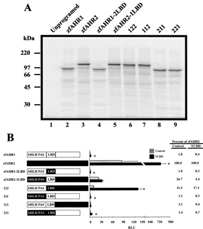
Fig. 12. Transactivation activity of chimeric zfAHRs in COS-7 cells. A, chimeric zfAHR1/zfAHR2 proteins were transcribed and translated in vitro in the presence of [ 35 S]methionine and resolved on an 8% SDS-PAGE gel. A phosphor image of the dried gel is shown; lanes include unprogrammed lysate (lane 1) and in vitro -expressed zfAHR1, zfAHR2, and chimeric zfAHRs (lanes 2–9). B, cells were transiently transfected with expression constructs for the indicated zfAHR construct along with zfARNT2b, a \beta -galactosidase reporter, and pGud-luc1.1 . Twenty-four hours after transfection, cells were exposed to 10 nM TCDD for 20 h followed by luciferase activity analysis. Bars represent the relative light units normalized to the \beta -galactosidase activity for DMSO (control) or TCDD (mean \pm S.E., n = 3 ). * indicates significant difference from DMSO control (Dunnett's test, p < 0.05 ).
